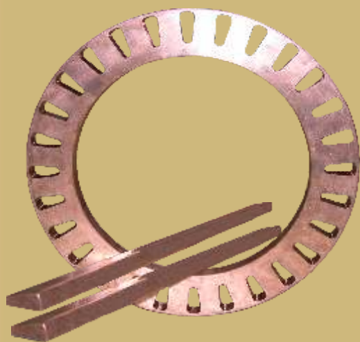
Short Circuit Ring & Rotor Bars for Traction Motors
