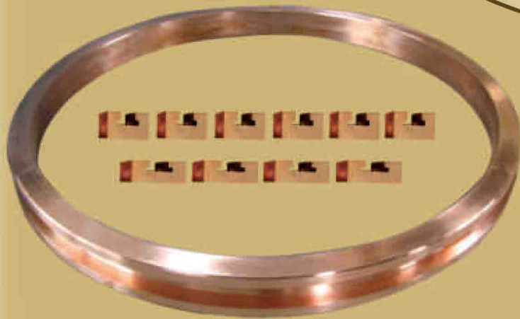
Casting Wheel & Dam blocks used for Continuous Cast Copper Rods (CCR) & Aluminium rods
